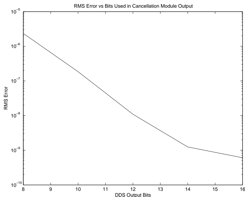
Figure 3.2: Effect of Quantization Noise on Cancellation
