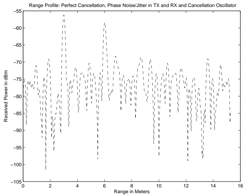
Figure 2.18: The radar range profile when phase noise is added to the transmit, receive and cancellation synthesizers
