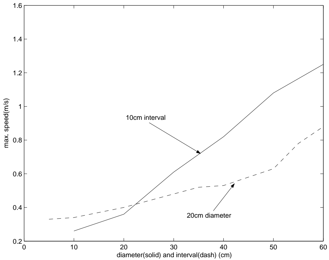
Figure 5.8: Speed at which radar moves up or down bore-hole
