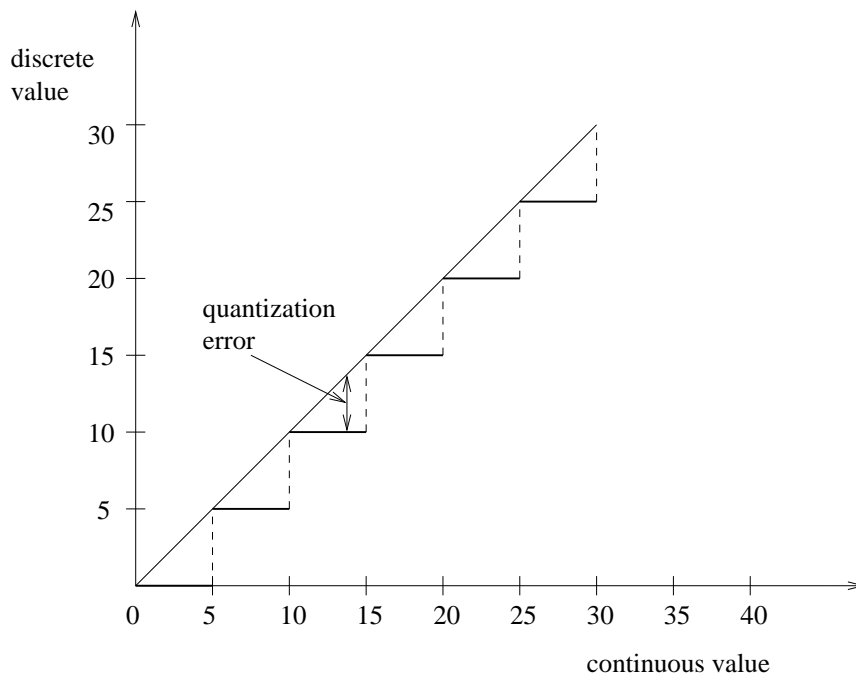
Figure 2.4: Digitization error
