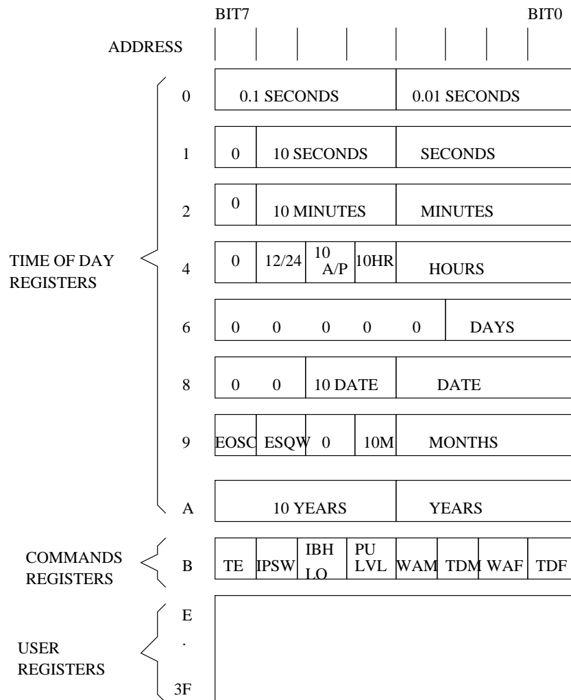
Figure 3.8: DS1286 registers
