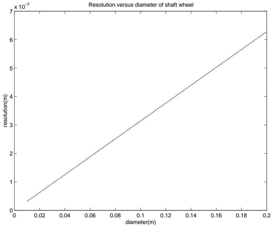
Figure 2.8: Resolution when CPR is 100
