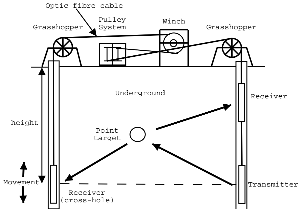
Figure 2.2: Geometry of bore-hole survey (with reference to [20])
