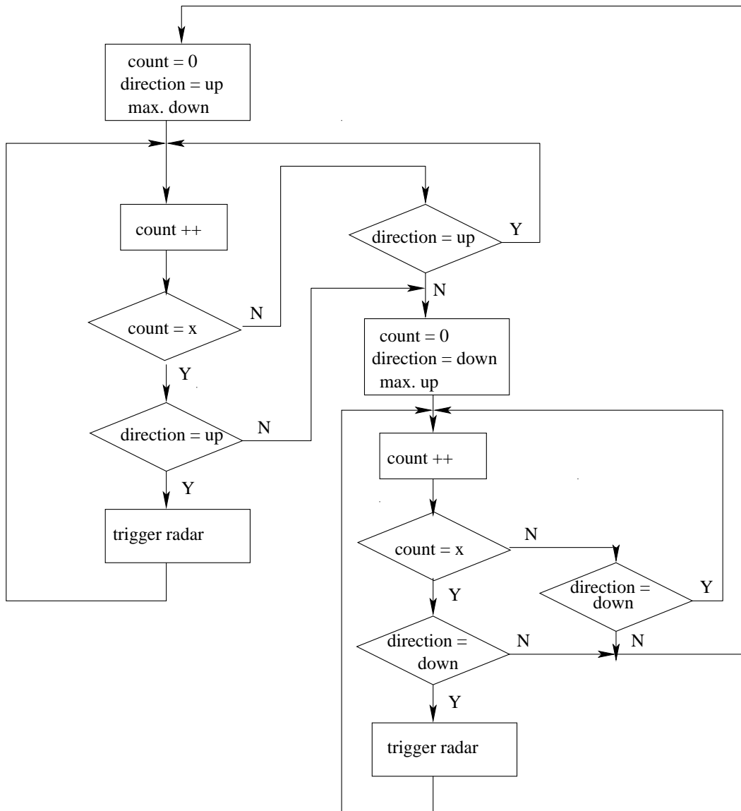
Figure 4.2: Flow chart for non timestamped data
