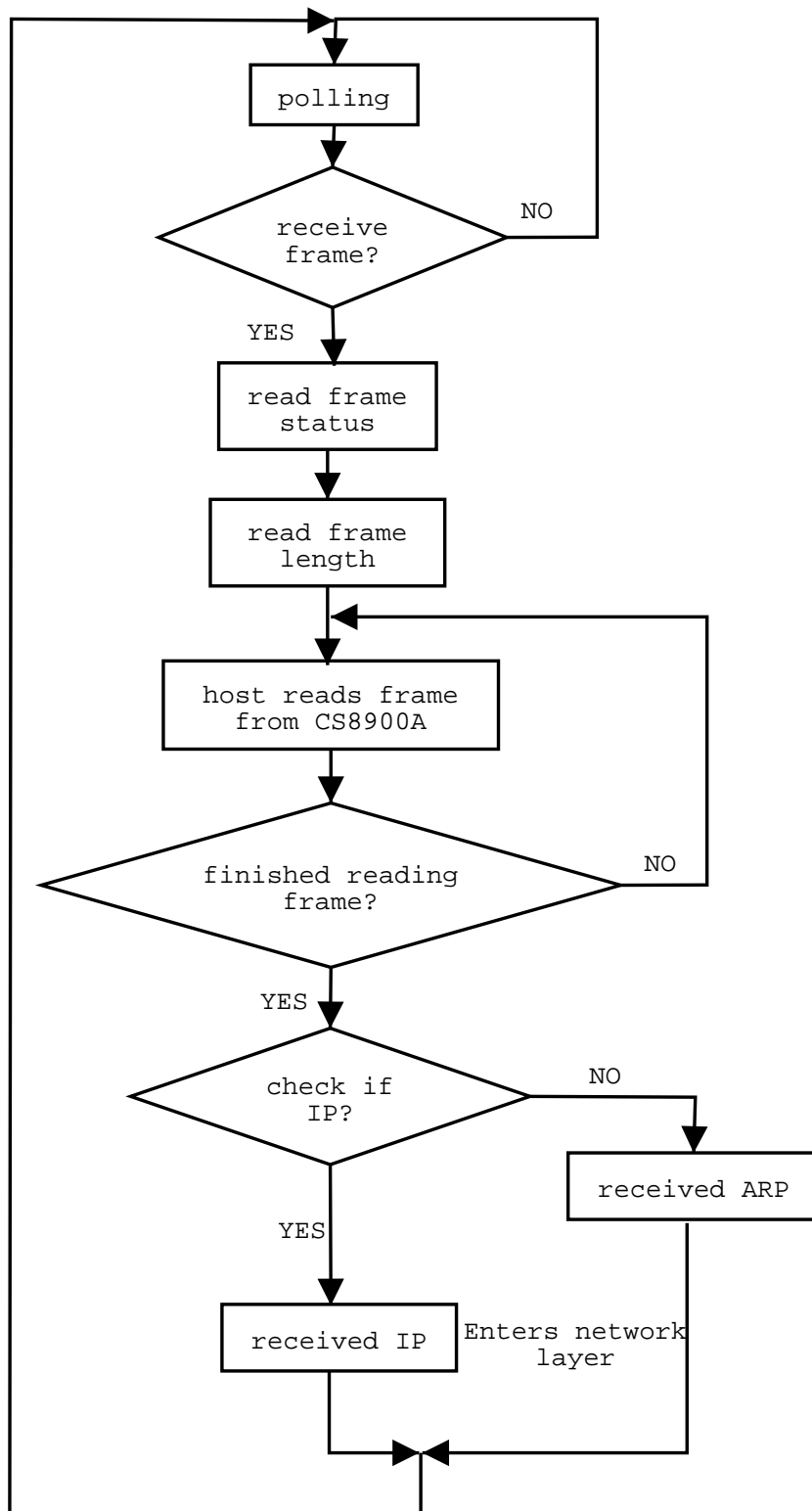
Figure 4.6: Polling mode
