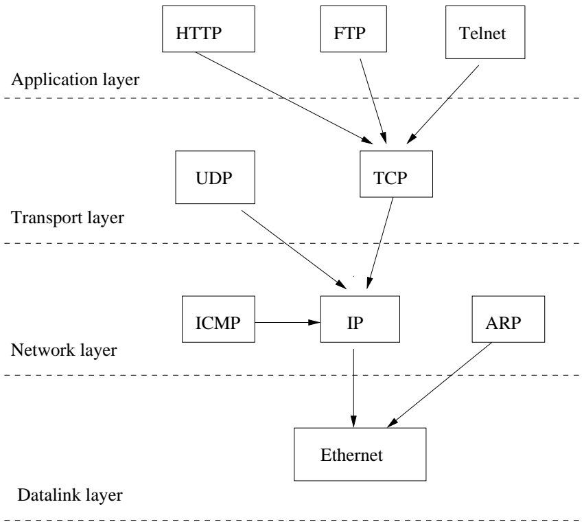
Figure 4.4: TCP/IP suite
