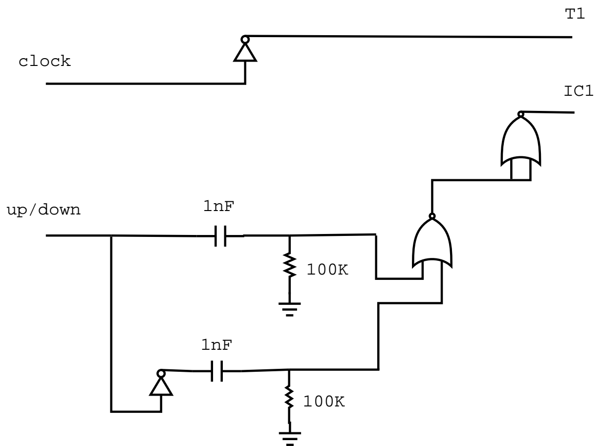
Figure 8.9: Circuit diagram of encoder to microcontroller interface
