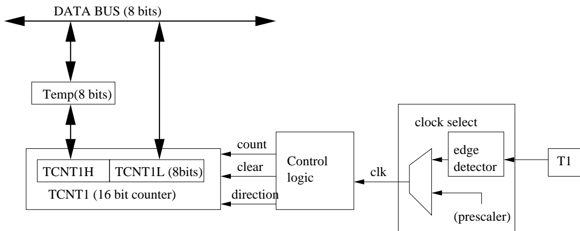
Figure 3.4: Counter unit (with reference to [10])
