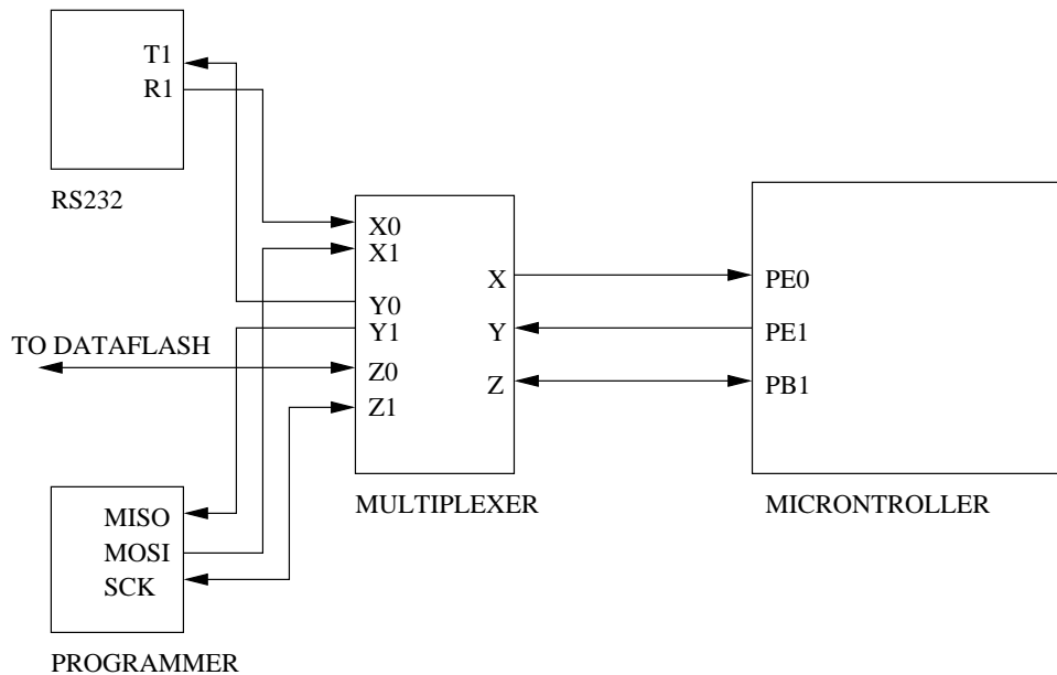
Figure 3.9: Serial interface
