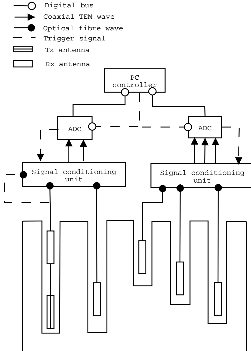
Figure 2.1: Block diagram of BHR (with reference to [20])
