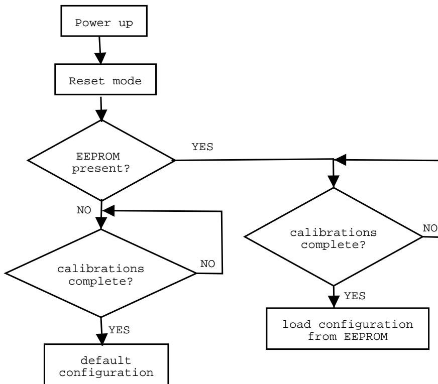
Figure 4.5: Initialization of CS8900A
