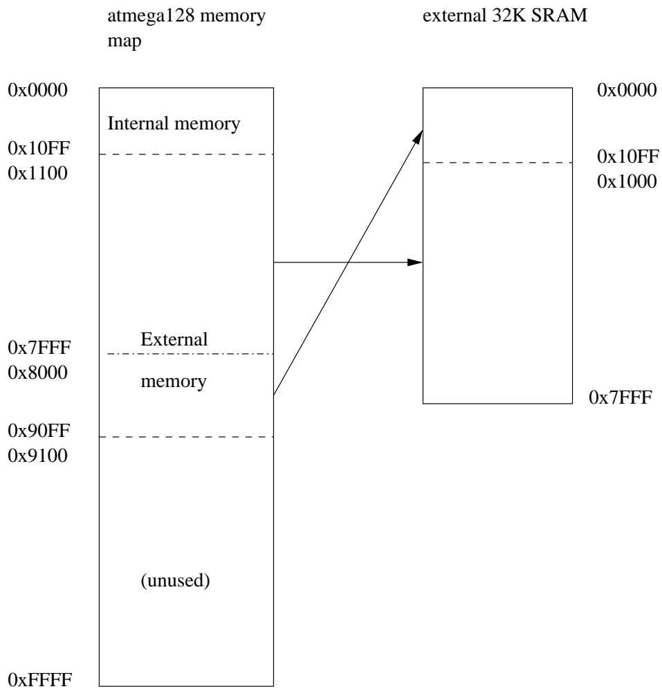
Figure 3.7: Atmega128 memory map(with reference to [10])
